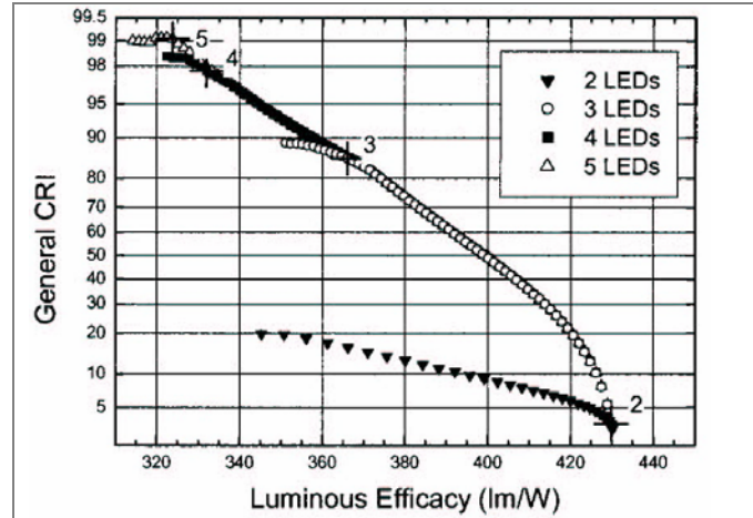
Figure 6. The envelope of maximum CRI and luminous efficacy for multi-LED white light sources with 30nm FWHM line widths and a 4870K color temperature. After A. Zukauskas, R. Vaicekauskas, F. Ivanauskas, R. Gaska, and M. S. Shur, "Optimization of white polychromatic semiconductor lamps," Applied Physics Letters 80 (2002) 234-6.
