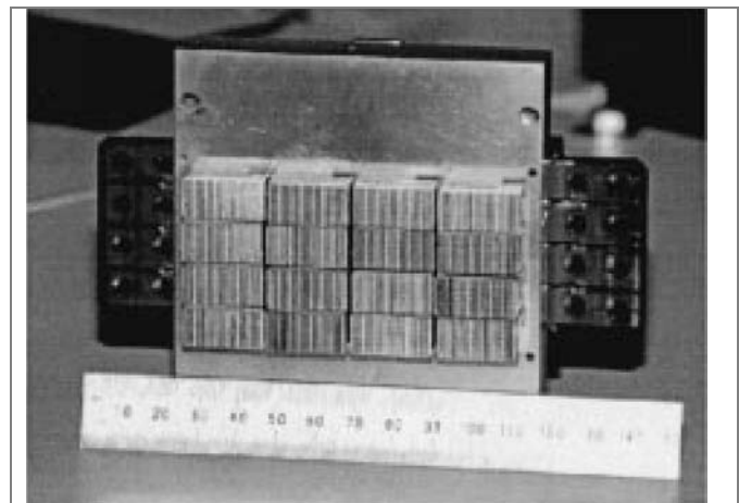
Figure 19. A 2D array of laser diode bars capable of 2.56kW average optical output power. If such powers were available in the three primary colors, the result would be roughly 1Mlm of white light. After D. F. Welch, "A Brief History of High-Power Semiconductor Lasers," IEEE Journal of Selected Topics in Quantum Electronics 6 (2000) 1470-1477.
