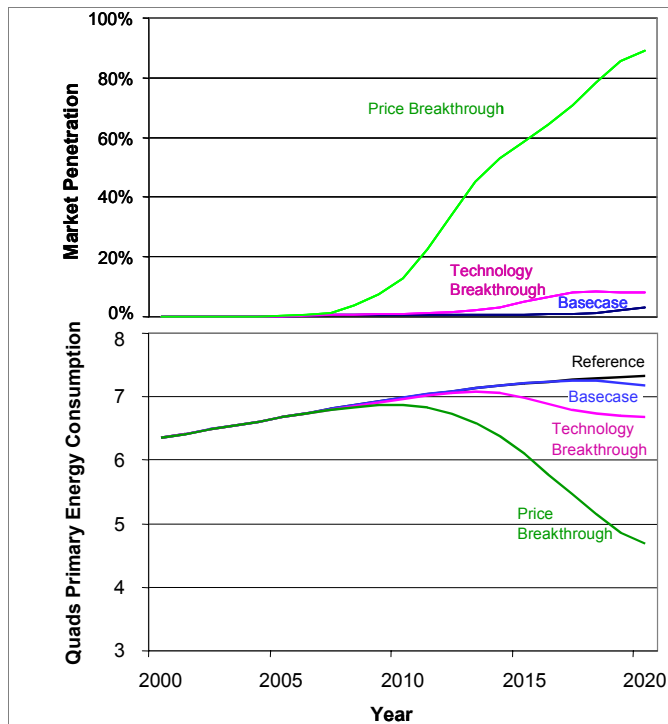
Figure 10. Market penetration and energy savings in both quads of primary energy and terawatt-hours of on-site electricity use. Note that these energy savings and market penetration estimates were based on a draft inventory of US lighting technologies. Estimates based on a revised lighting inventory are expected to be available in early 2003. Mark Kendall and Michael Scholand, "Energy Savings Potential of Solid State Lighting in General Lighting Applications" (U.S. Department of Energy, Office of Building Technology, State and Community Programs, Apr, 2001).
